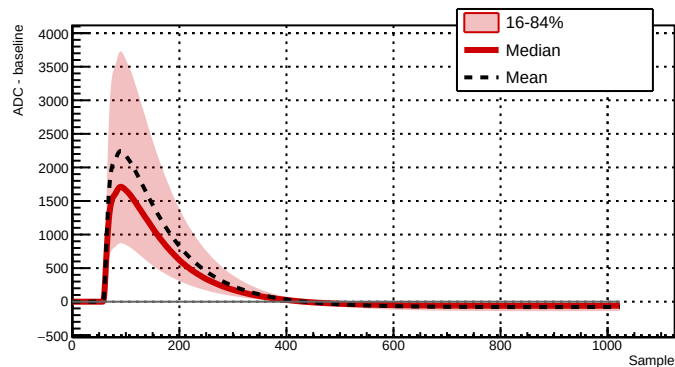
Run 039506 - Channel 2081 - 27996 waveforms
