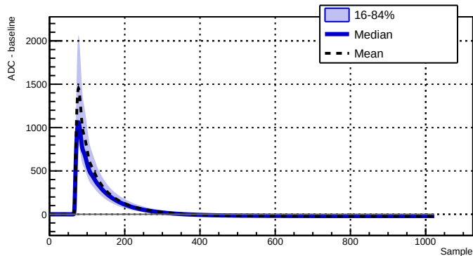
Run 039506 - Channel 2070 - 11176 waveforms
