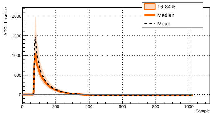
Run 039506 - Channel 2071 - 10765 waveforms
