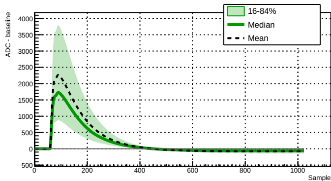
Run 039506 - Channel 2080 - 27525 waveforms
