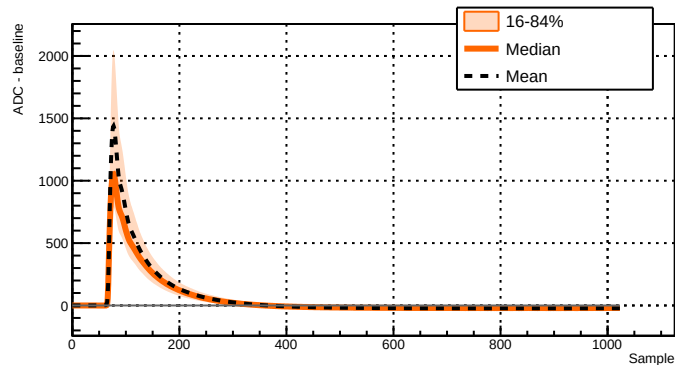
Run 039507 - Channel 2071 - 11470 waveforms
