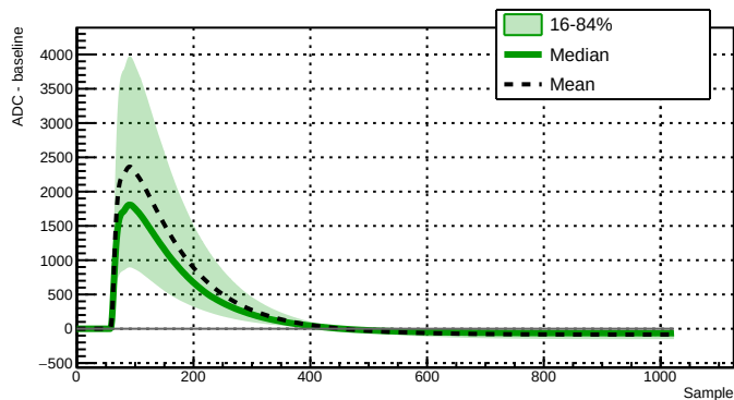
Run 039507 - Channel 2080 - 28726 waveforms
