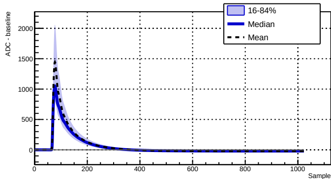
Run 039507 - Channel 2070 - 11985 waveforms
