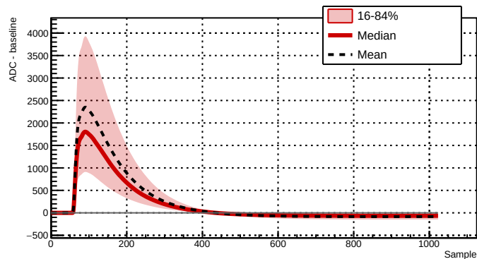
Run 039507 - Channel 2081 - 29138 waveforms
