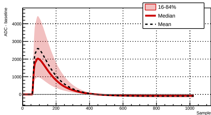
Run 039511 - Channel 2081 - 30507 waveforms
