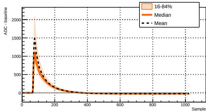
Run 039511 - Channel 2071 - 13191 waveforms
