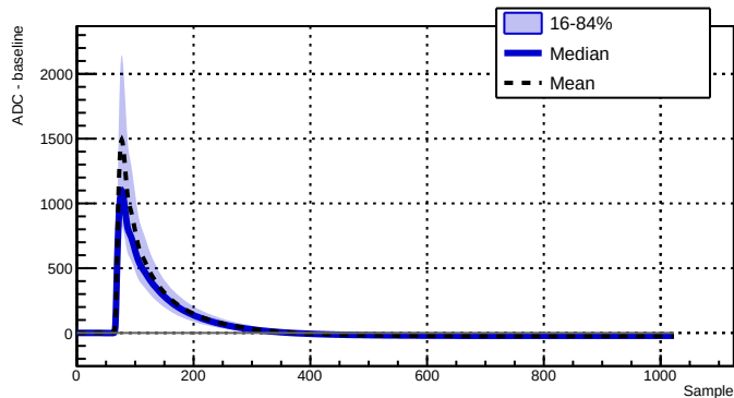
Run 039511 - Channel 2070 - 13639 waveforms
