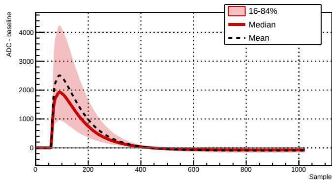
Run 039512 - Channel 2081 - 29826 waveforms
