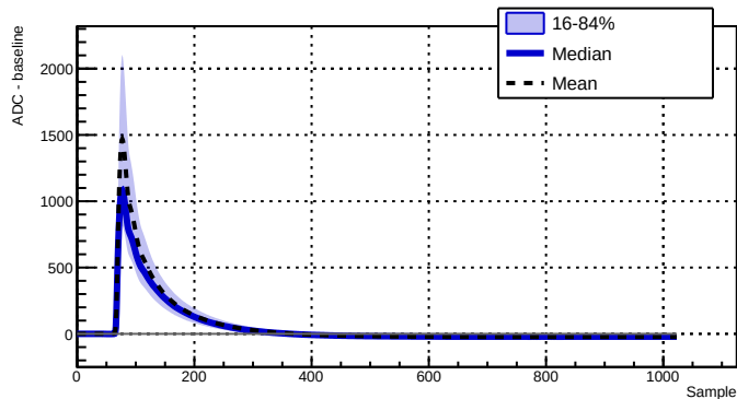
Run 039512 - Channel 2070 - 12932 waveforms
