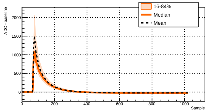
Run 039512 - Channel 2071 - 12551 waveforms
