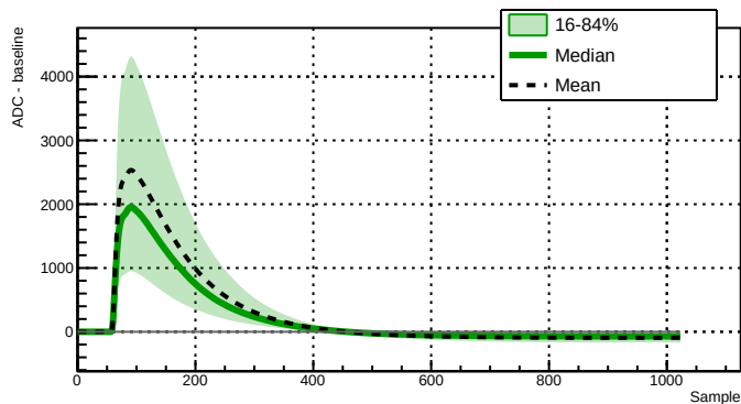
Run 039512 - Channel 2080 - 29175 waveforms
