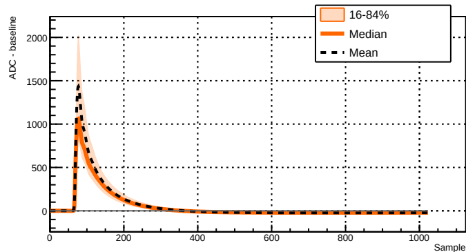
Run 039514 - Channel 2071 - 11837 waveforms
