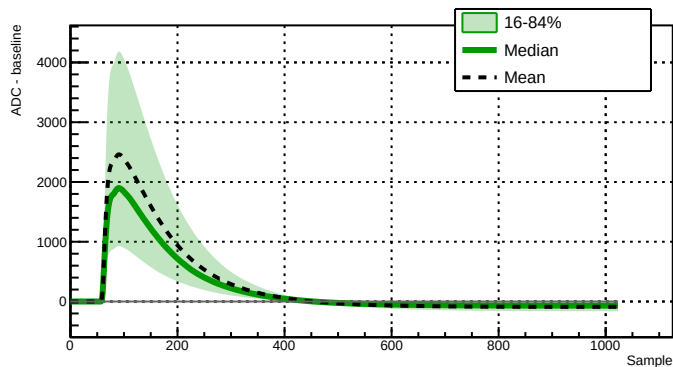
Run 039514 - Channel 2080 - 28493 waveforms
