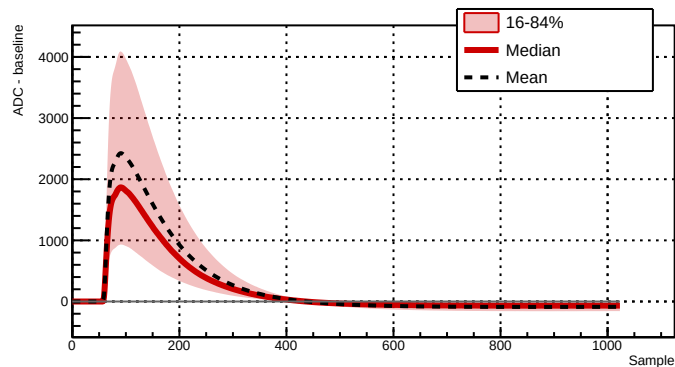
Run 039514 - Channel 2081 - 29001 waveforms
