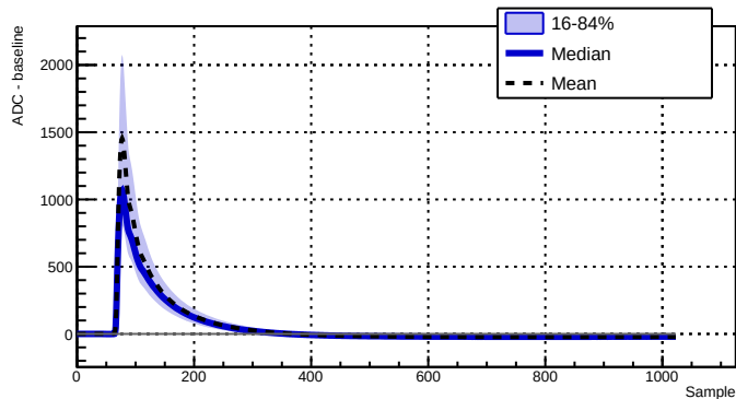
Run 039514 - Channel 2070 - 12217 waveforms
