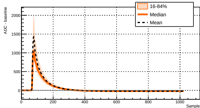
Run 039516 - Channel 2071 - 10859 waveforms
