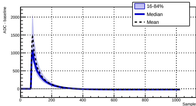
Run 039517 - Channel 2070 - 11002 waveforms
