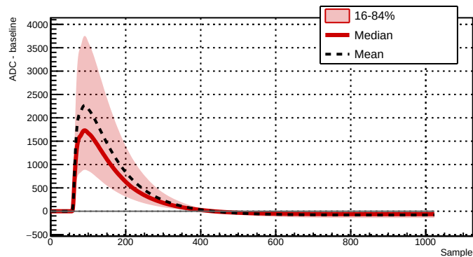
Run 039517 - Channel 2081 - 27658 waveforms
