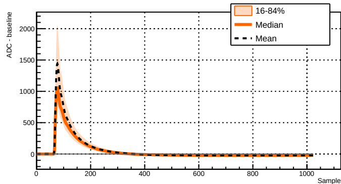
Run 039517 - Channel 2071 - 10634 waveforms
