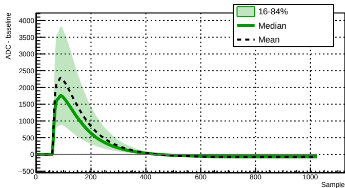
Run 039517 - Channel 2080 - 27175 waveforms
