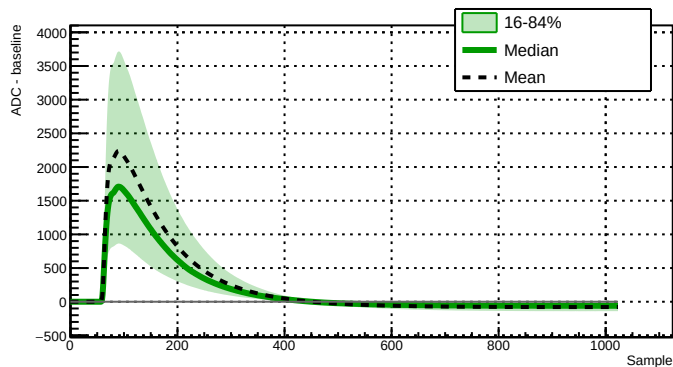
Run 039518 - Channel 2080 - 26824 waveforms
