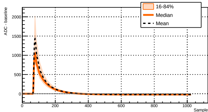
Run 039518 - Channel 2071 - 10329 waveforms
