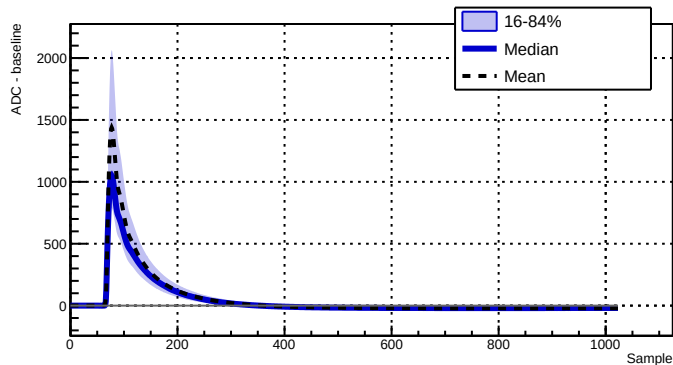
Run 039518 - Channel 2070 - 10632 waveforms
