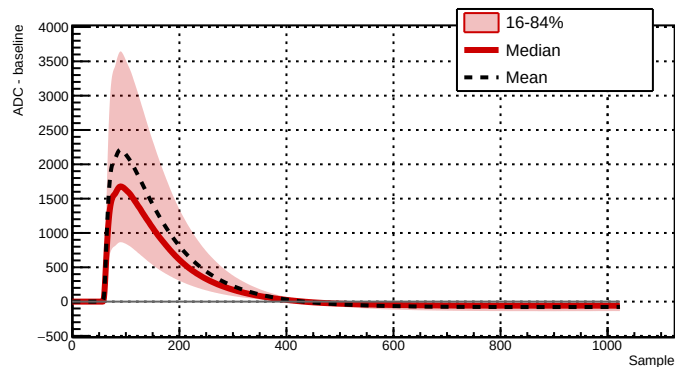
Run 039518 - Channel 2081 - 27291 waveforms
