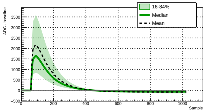
Run 039519 - Channel 2080 - 26694 waveforms
