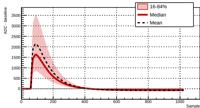
Run 039519 - Channel 2081 - 26912 waveforms
