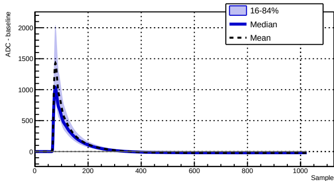
Run 039519 - Channel 2070 - 10449 waveforms
