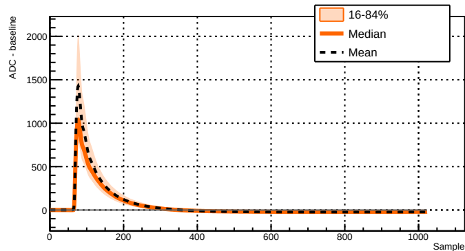
Run 039519 - Channel 2071 - 10007 waveforms
