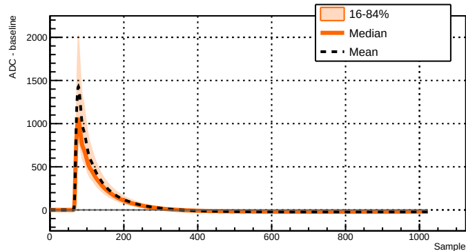
Run 039521 - Channel 2071 - 9545 waveforms
