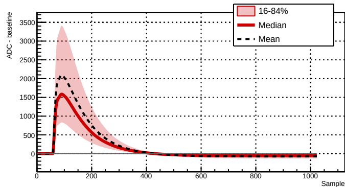
Run 039521 - Channel 2081 - 26062 waveforms
