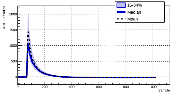
Run 039521 - Channel 2070 - 9985 waveforms
