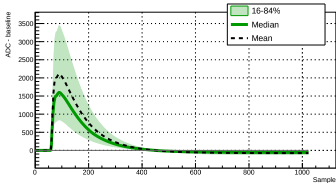
Run 039521 - Channel 2080 - 25846 waveforms
