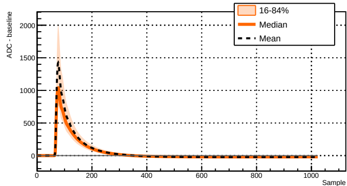
Run 039522 - Channel 2071 - 9410 waveforms
