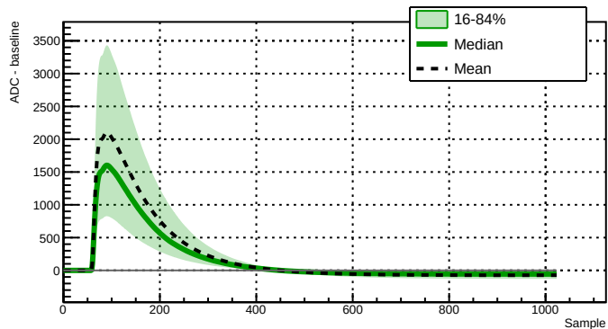
Run 039522 - Channel 2080 - 25553 waveforms
