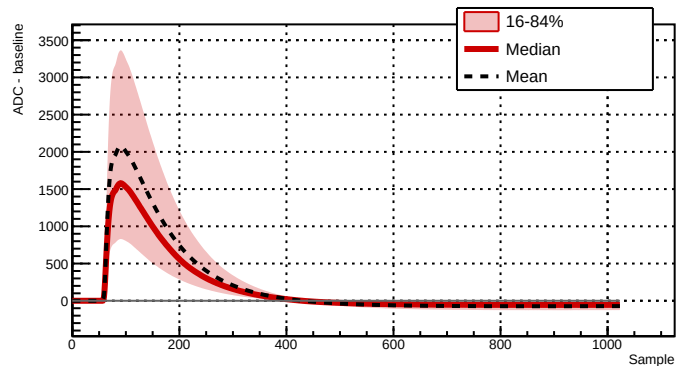
Run 039522 - Channel 2081 - 25882 waveforms
