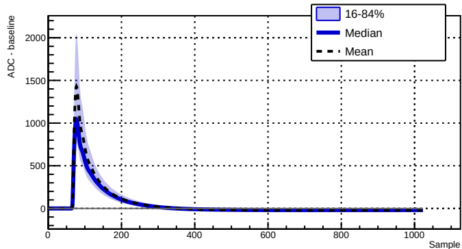
Run 039522 - Channel 2070 - 9845 waveforms
