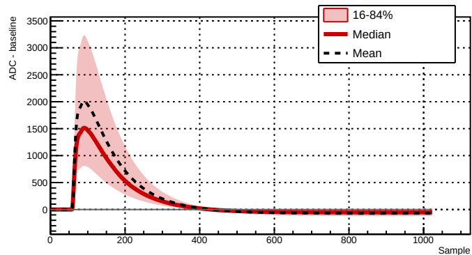
Run 039523 - Channel 2081 - 25252 waveforms
