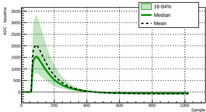
Run 039523 - Channel 2080 - 25008 waveforms
