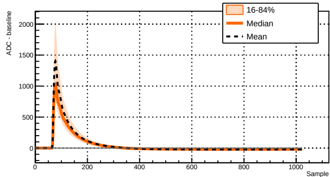
Run 039523 - Channel 2071 - 9085 waveforms
