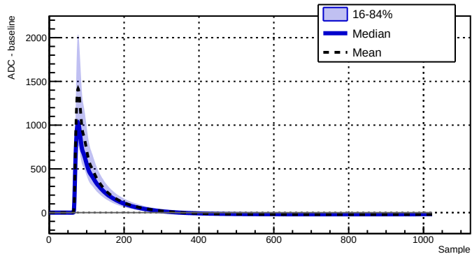
Run 039523 - Channel 2070 - 9454 waveforms
