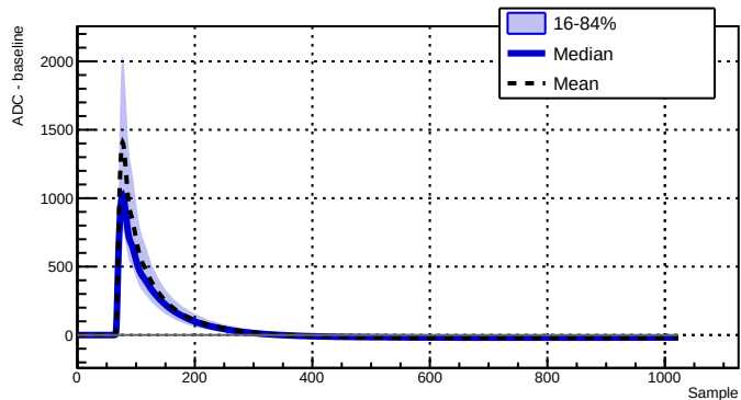
Run 039527 - Channel 2070 - 8806 waveforms
