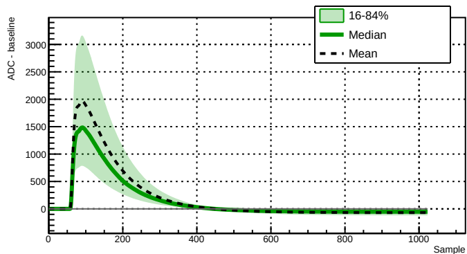
Run 039527 - Channel 2080 - 24168 waveforms
