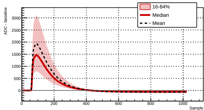
Run 039527 - Channel 2081 - 24292 waveforms
