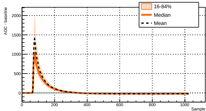
Run 039527 - Channel 2071 - 8511 waveforms
