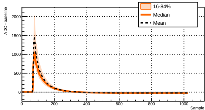
Run 039529 - Channel 2071 - 7920 waveforms
