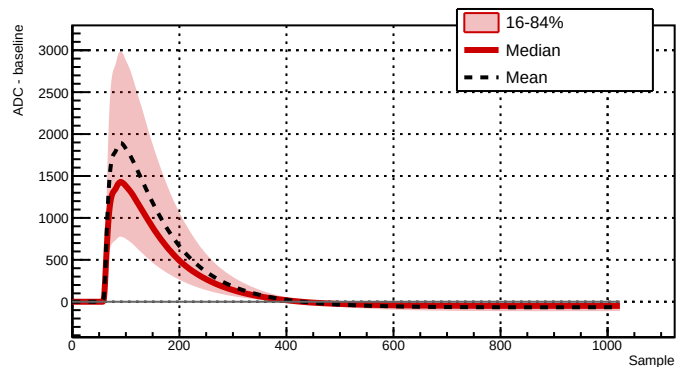
Run 039529 - Channel 2081 - 23818 waveforms
