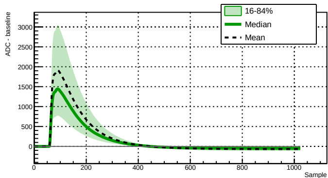
Run 039529 - Channel 2080 - 23600 waveforms
