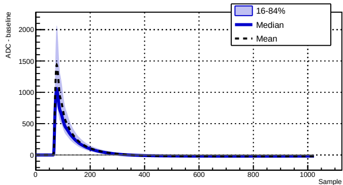
Run 039529 - Channel 2070 - 8226 waveforms
