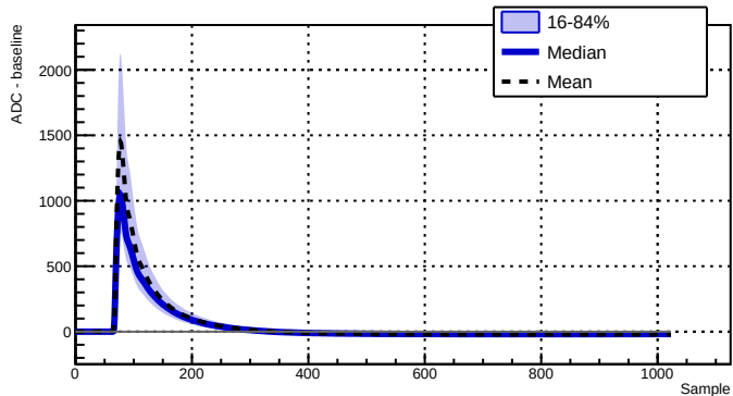
Run 041523 - Channel 2070 - 5811 waveforms
