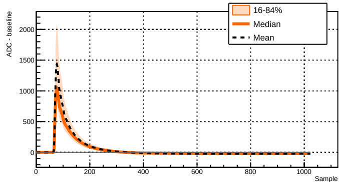
Run 041523 - Channel 2071 - 5622 waveforms
