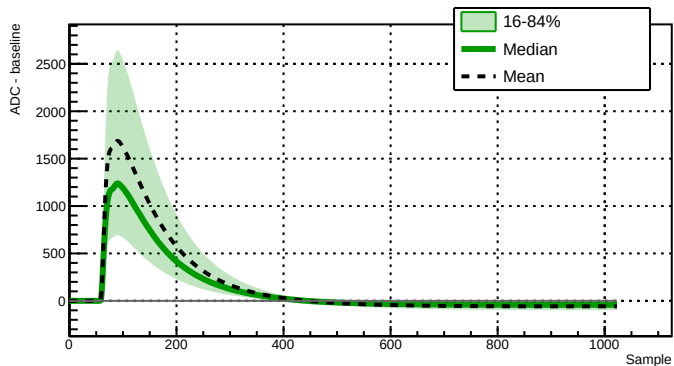
Run 041523 - Channel 2080 - 17906 waveforms
