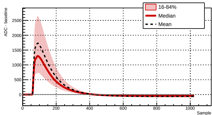
Run 043380 - Channel 2081 - 18814 waveforms
