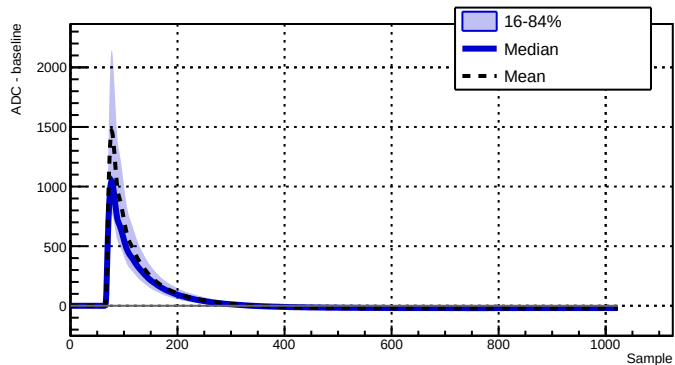
Run 043380 - Channel 2070 - 6154 waveforms
