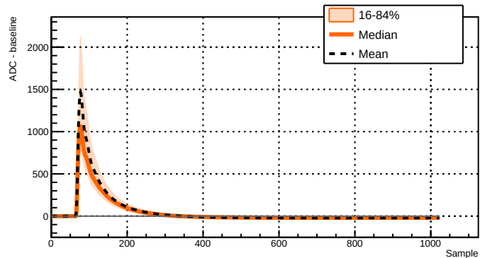
Run 043380 - Channel 2071 - 5867 waveforms
