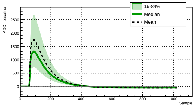
Run 043380 - Channel 2080 - 18743 waveforms
