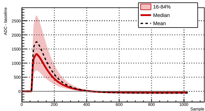
Run 043381 - Channel 2081 - 18779 waveforms
