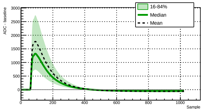
Run 043381 - Channel 2080 - 18807 waveforms
