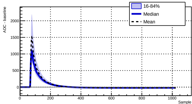
Run 043381 - Channel 2070 - 5968 waveforms
