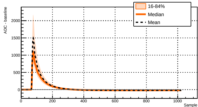
Run 043381 - Channel 2071 - 5726 waveforms
