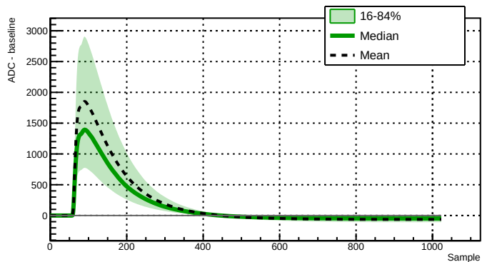
Run 043383 - Channel 2080 - 19452 waveforms
