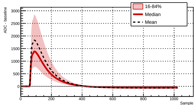
Run 043383 - Channel 2081 - 19493 waveforms
