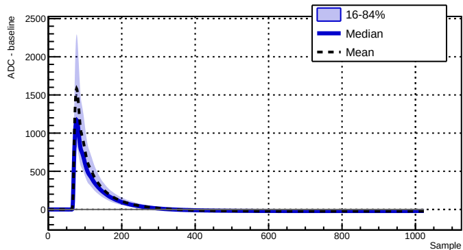
Run 043383 - Channel 2070 - 6212 waveforms
