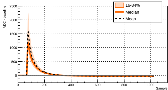
Run 043383 - Channel 2071 - 5922 waveforms
