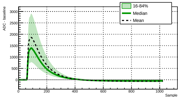
Run 043384 - Channel 2080 - 19519 waveforms
