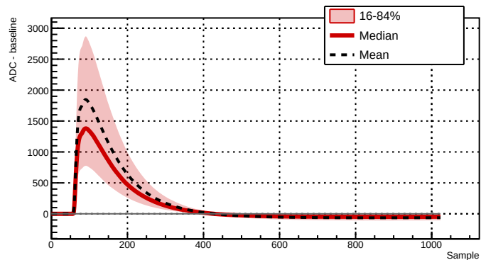
Run 043384 - Channel 2081 - 19696 waveforms
