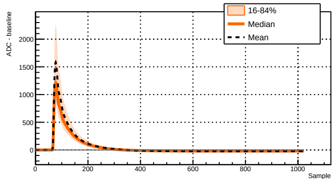
Run 043384 - Channel 2071 - 6112 waveforms
