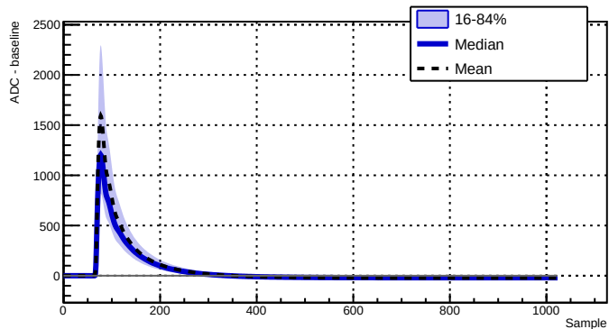
Run 043384 - Channel 2070 - 6306 waveforms
