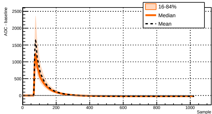
Run 043386 - Channel 2071 - 5386 waveforms
