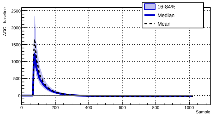
Run 043386 - Channel 2070 - 5662 waveforms
