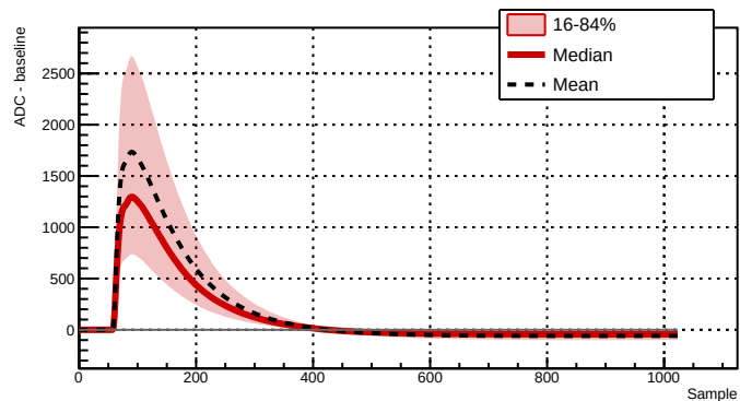
Run 043386 - Channel 2081 - 18129 waveforms
