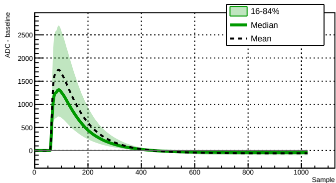
Run 043386 - Channel 2080 - 18153 waveforms
