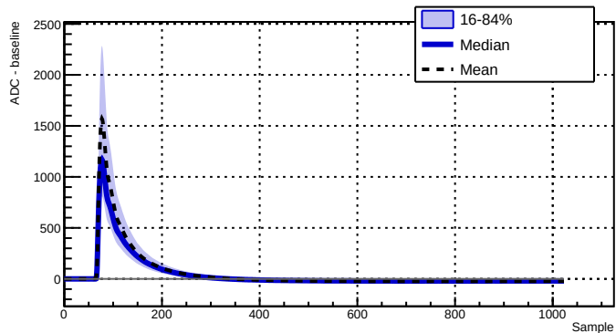
Run 043387 - Channel 2070 - 5504 waveforms
