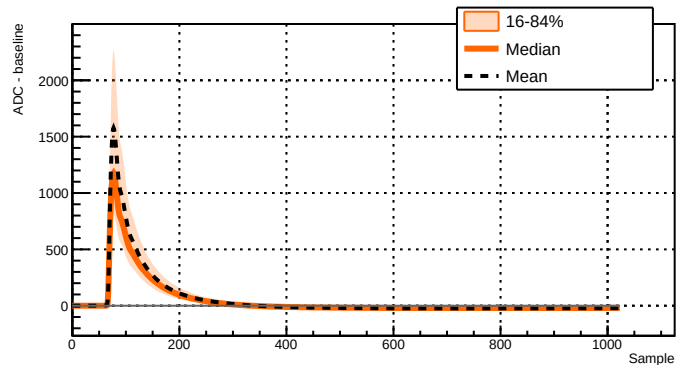
Run 043387 - Channel 2071 - 5270 waveforms
