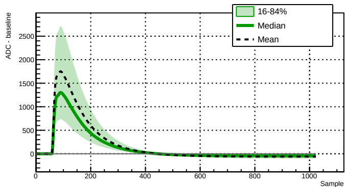
Run 043387 - Channel 2080 - 18213 waveforms
