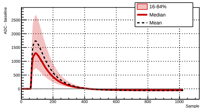
Run 043387 - Channel 2081 - 18200 waveforms
