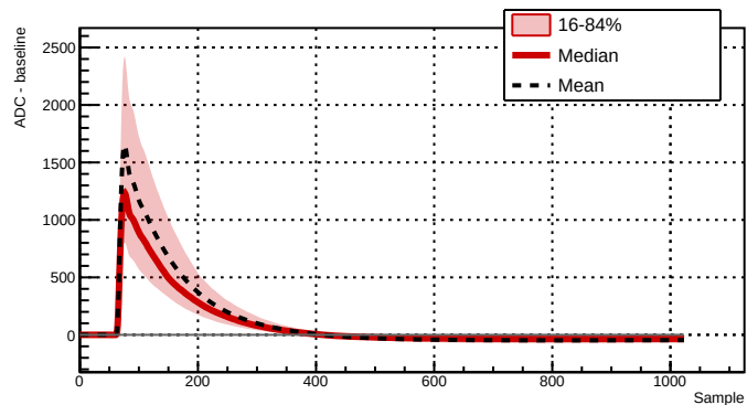
Run 039501 - Channel 2061 - 5793 waveforms
