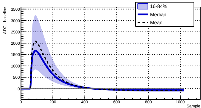
Run 039501 - Channel 2050 - 8852 waveforms
