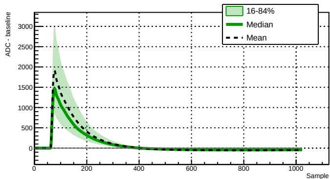
Run 039501 - Channel 2060 - 7044 waveforms
