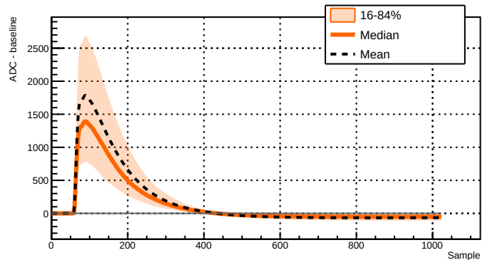
Run 039501 - Channel 2051 - 7320 waveforms
