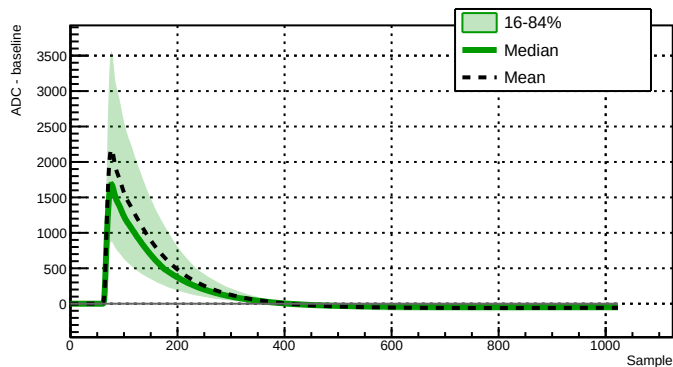
Run 039504 - Channel 2060 - 7825 waveforms
