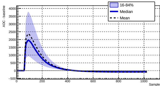
Run 039504 - Channel 2050 - 10202 waveforms
