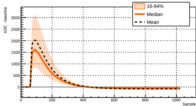
Run 039504 - Channel 2051 - 8586 waveforms
