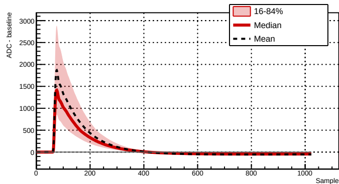
Run 039504 - Channel 2061 - 6253 waveforms
