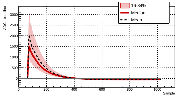
Run 039506 - Channel 2061 - 6678 waveforms
