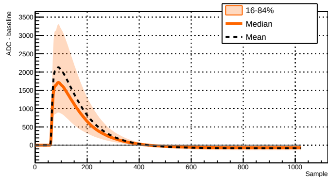
Run 039506 - Channel 2051 - 8918 waveforms
