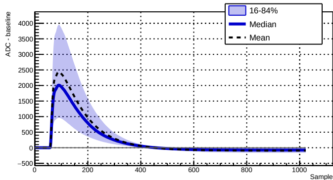
Run 039506 - Channel 2050 - 11060 waveforms
