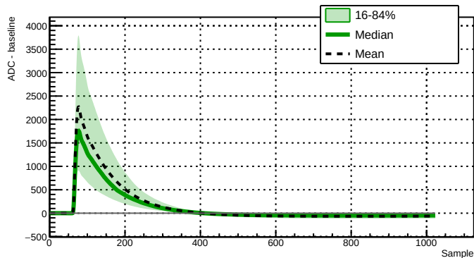
Run 039506 - Channel 2060 - 8290 waveforms
