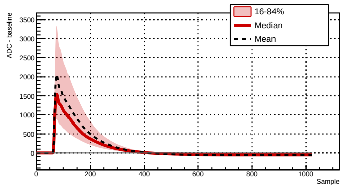
Run 039507 - Channel 2061 - 6948 waveforms
