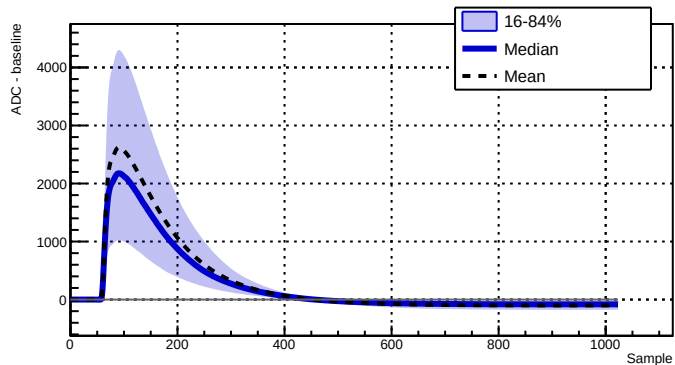
Run 039507 - Channel 2050 - 11768 waveforms
