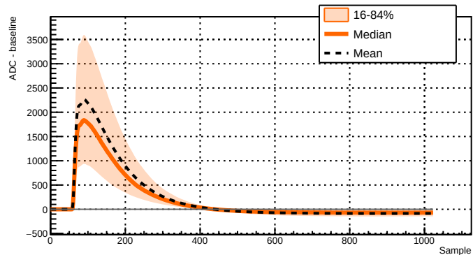
Run 039507 - Channel 2051 - 9746 waveforms
