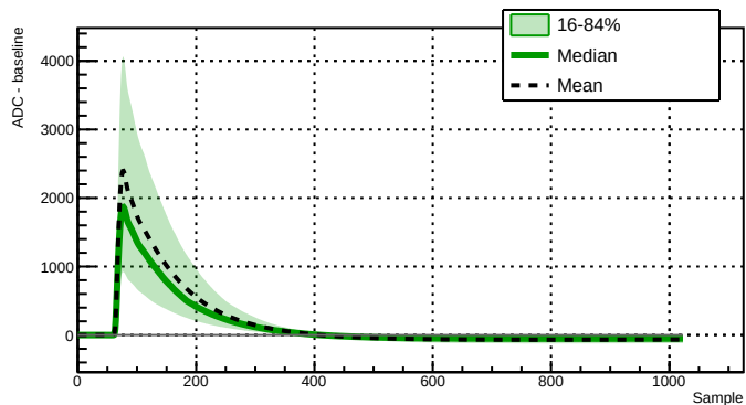
Run 039507 - Channel 2060 - 8889 waveforms
