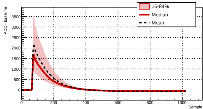
Run 039508 - Channel 2061 - 7045 waveforms
