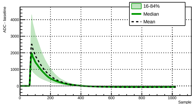
Run 039508 - Channel 2060 - 8927 waveforms
