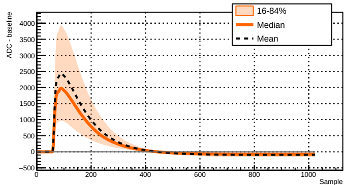
Run 039508 - Channel 2051 - 10238 waveforms
