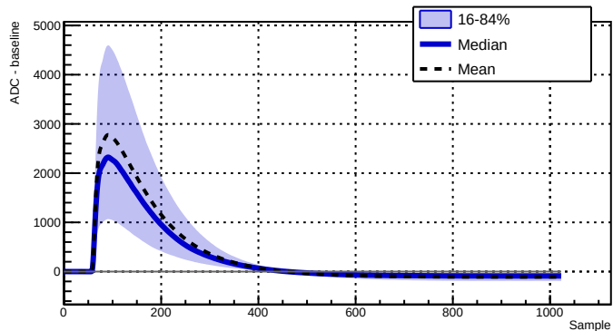
Run 039508 - Channel 2050 - 12366 waveforms
