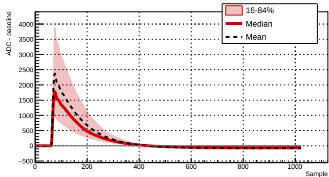
Run 039510 - Channel 2061 - 6035 waveforms
