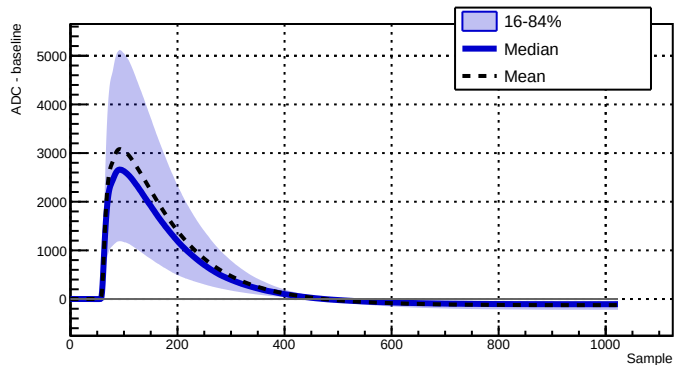
Run 039510 - Channel 2050 - 12138 waveforms
