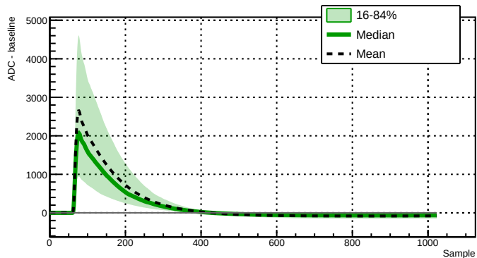
Run 039510 - Channel 2060 - 7926 waveforms
