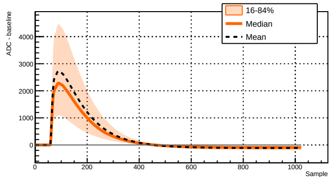
Run 039510 - Channel 2051 - 10036 waveforms
