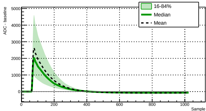
Run 039511 - Channel 2060 - 9347 waveforms
