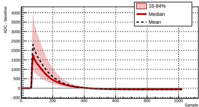
Run 039511 - Channel 2061 - 7077 waveforms
