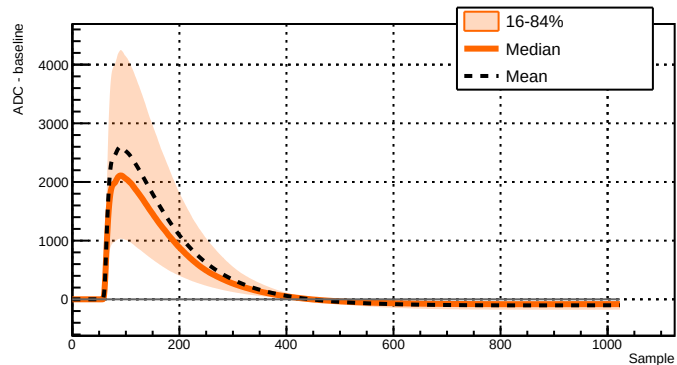
Run 039511 - Channel 2051 - 10711 waveforms
