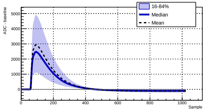
Run 039511 - Channel 2050 - 13037 waveforms
