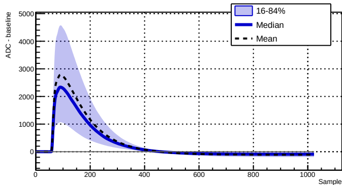
Run 039512 - Channel 2050 - 12622 waveforms
