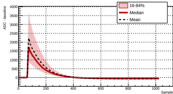
Run 039512 - Channel 2061 - 7147 waveforms
