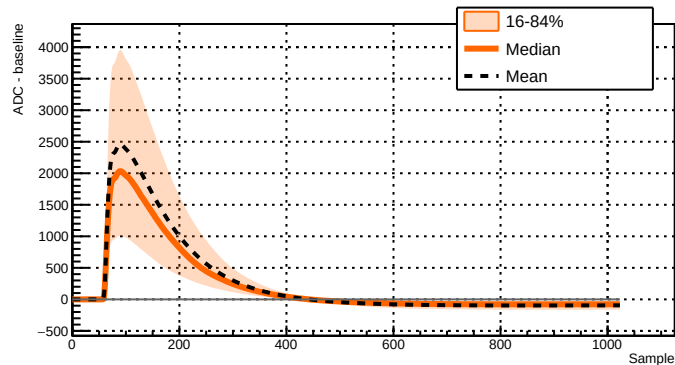
Run 039512 - Channel 2051 - 10426 waveforms
