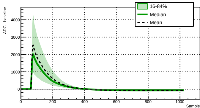
Run 039512 - Channel 2060 - 9153 waveforms
