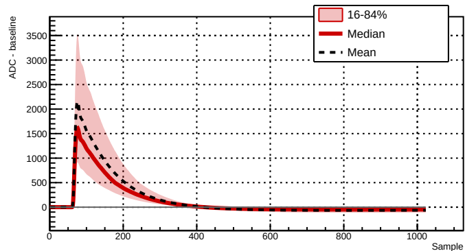
Run 039514 - Channel 2061 - 7078 waveforms
