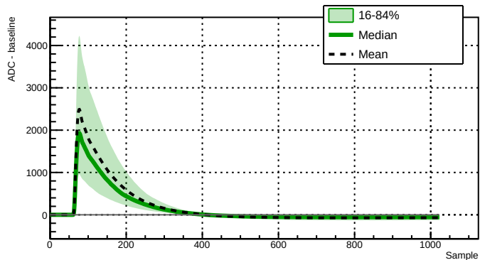
Run 039514 - Channel 2060 - 8596 waveforms
