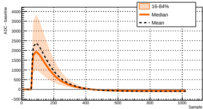
Run 039514 - Channel 2051 - 9977 waveforms
