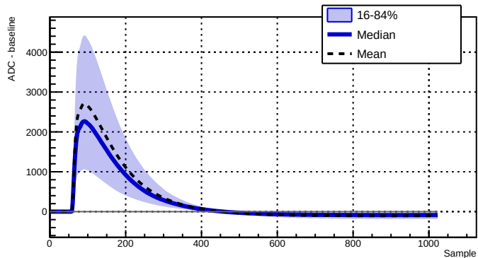
Run 039514 - Channel 2050 - 12030 waveforms
