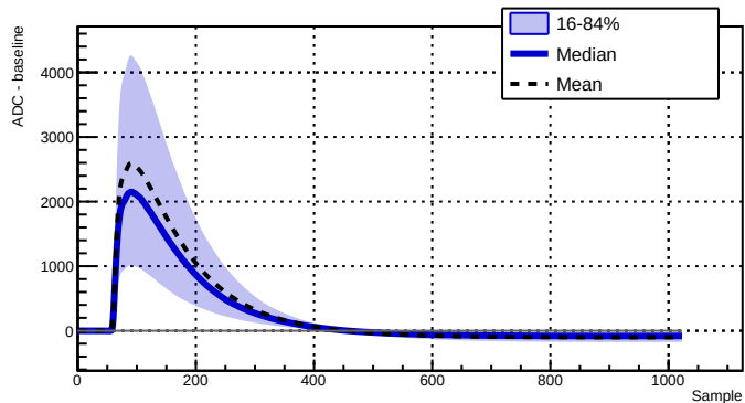
Run 039515 - Channel 2050 - 11612 waveforms
