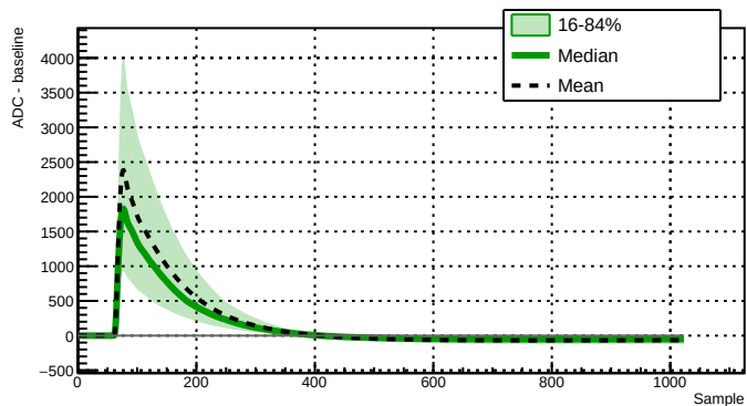
Run 039515 - Channel 2060 - 8501 waveforms
