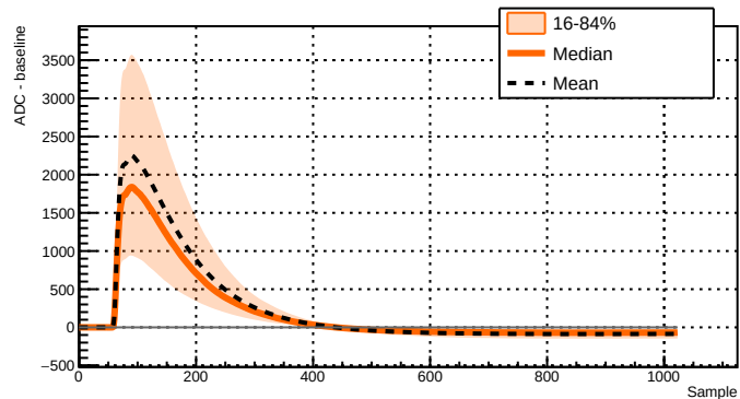
Run 039515 - Channel 2051 - 9528 waveforms
