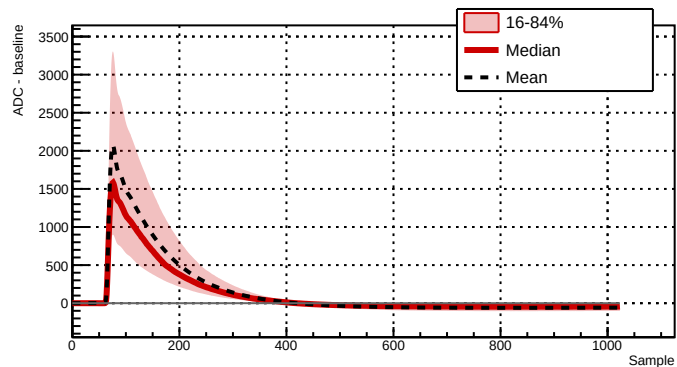
Run 039515 - Channel 2061 - 6722 waveforms
