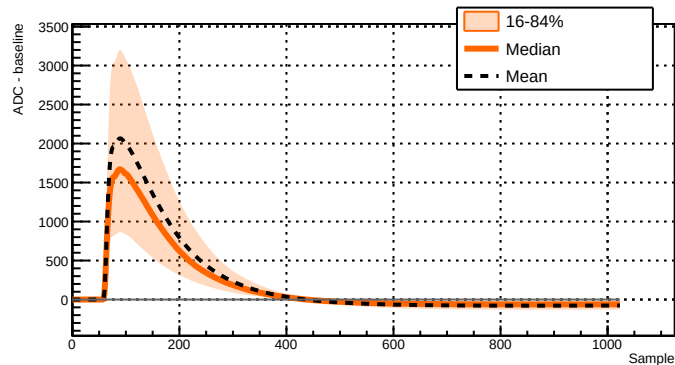
Run 039518 - Channel 2051 - 8699 waveforms
