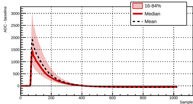
Run 039518 - Channel 2061 - 6466 waveforms
