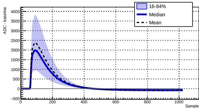
Run 039518 - Channel 2050 - 10539 waveforms
