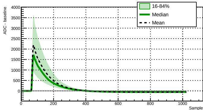
Run 039518 - Channel 2060 - 8164 waveforms
