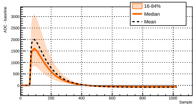
Run 039519 - Channel 2051 - 8592 waveforms
