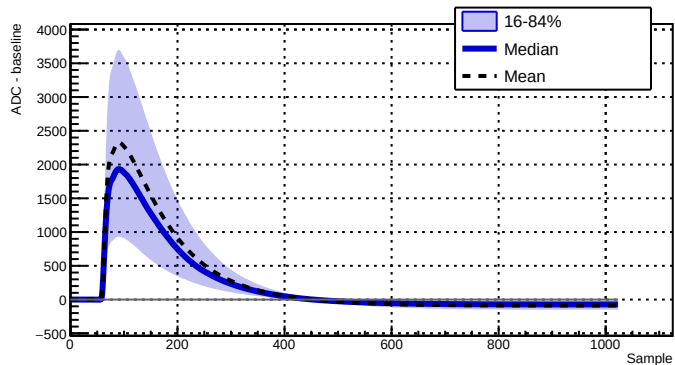
Run 039519 - Channel 2050 - 10265 waveforms
