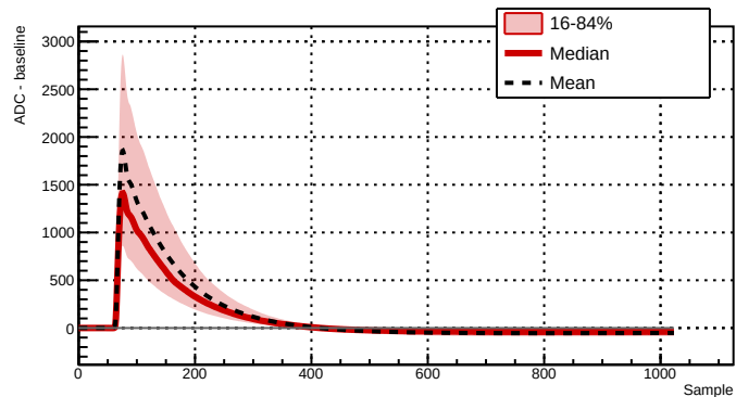
Run 039519 - Channel 2061 - 6388 waveforms
