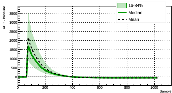
Run 039519 - Channel 2060 - 7969 waveforms
