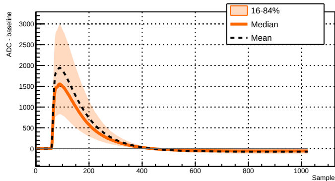
Run 039521 - Channel 2051 - 8194 waveforms
