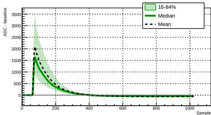
Run 039521 - Channel 2060 - 7833 waveforms
