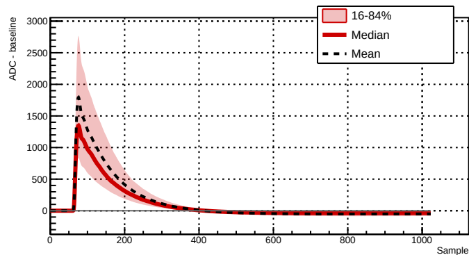
Run 039521 - Channel 2061 - 6233 waveforms
