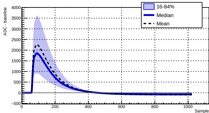
Run 039521 - Channel 2050 - 10017 waveforms
