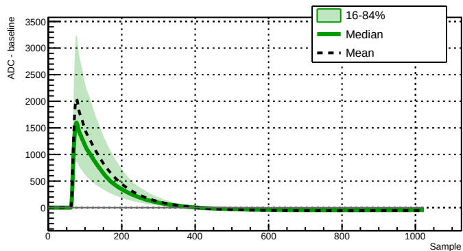
Run 039522 - Channel 2060 - 7623 waveforms
