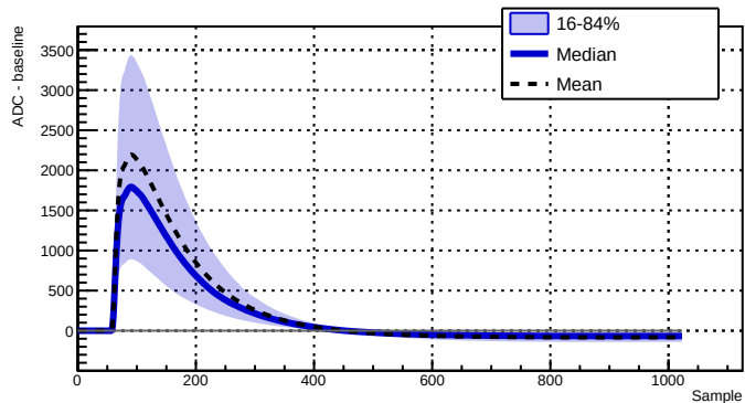
Run 039522 - Channel 2050 - 9681 waveforms
