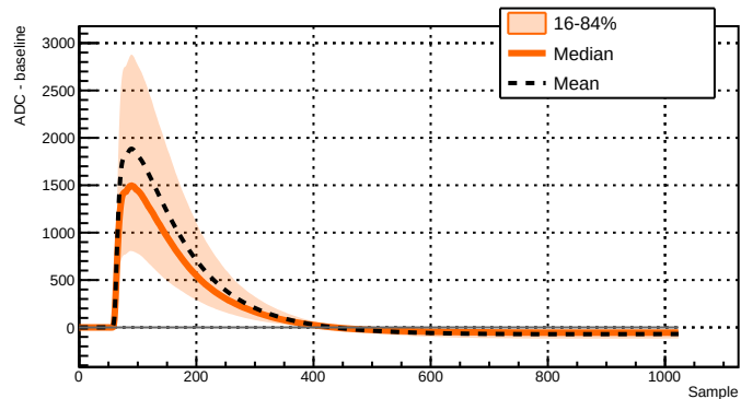
Run 039522 - Channel 2051 - 7942 waveforms
