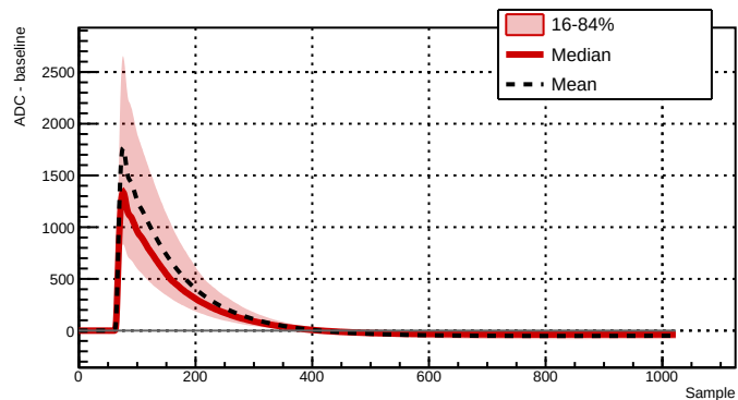
Run 039522 - Channel 2061 - 6021 waveforms
