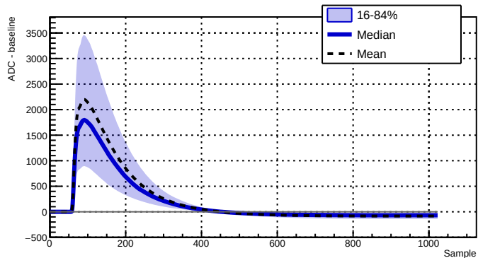
Run 039523 - Channel 2050 - 9462 waveforms
