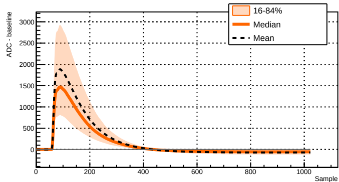
Run 039523 - Channel 2051 - 7640 waveforms
