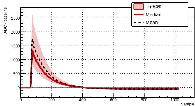
Run 039523 - Channel 2061 - 6133 waveforms
