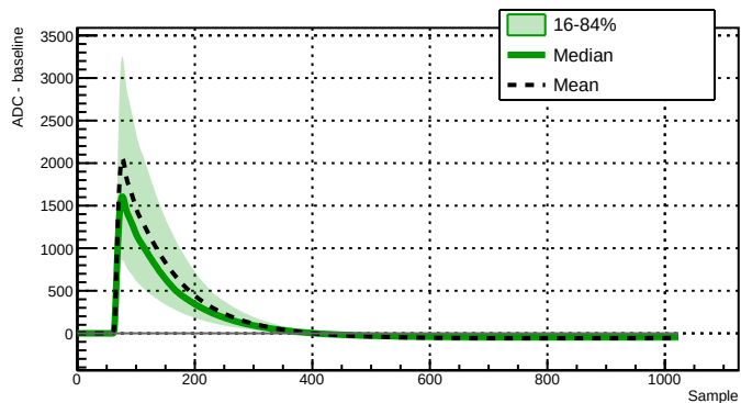
Run 039523 - Channel 2060 - 7505 waveforms
