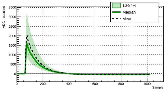
Run 039525 - Channel 2060 - 7337 waveforms
