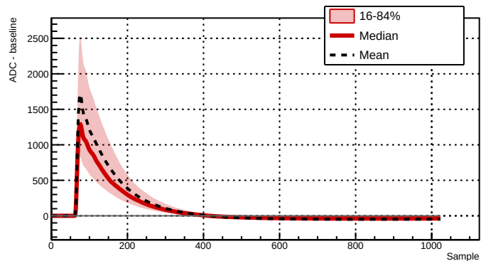
Run 039525 - Channel 2061 - 5959 waveforms
