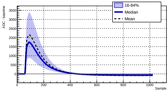
Run 039525 - Channel 2050 - 9232 waveforms
