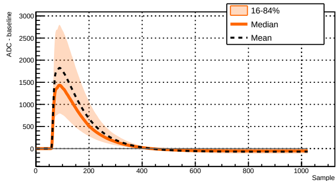
Run 039525 - Channel 2051 - 7564 waveforms
