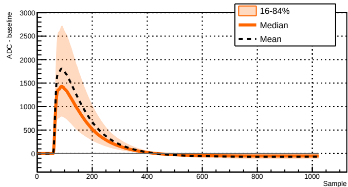
Run 039526 - Channel 2051 - 7444 waveforms
