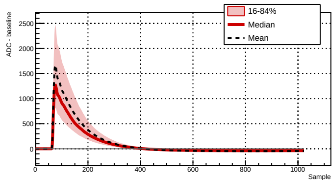
Run 039526 - Channel 2061 - 5887 waveforms
