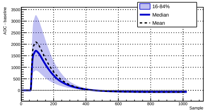
Run 039526 - Channel 2050 - 9141 waveforms
