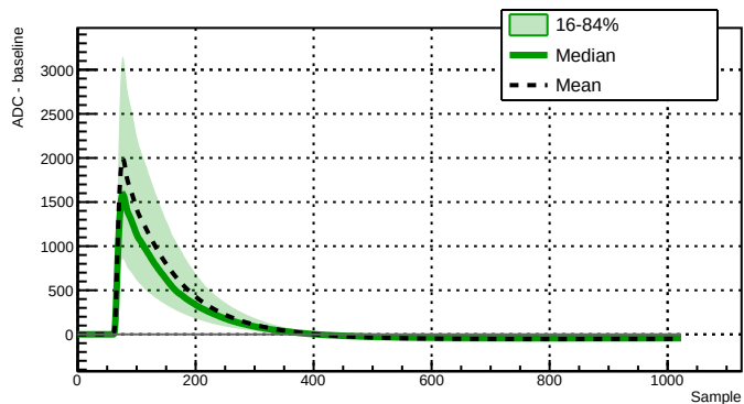
Run 039526 - Channel 2060 - 7202 waveforms
