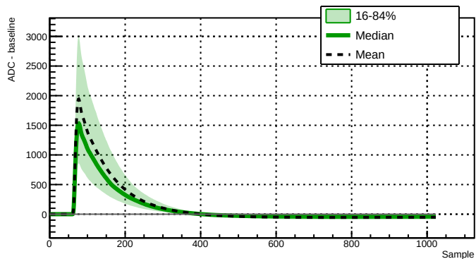
Run 039527 - Channel 2060 - 7084 waveforms
