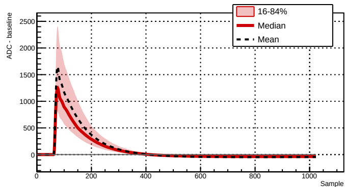
Run 039527 - Channel 2061 - 5733 waveforms
