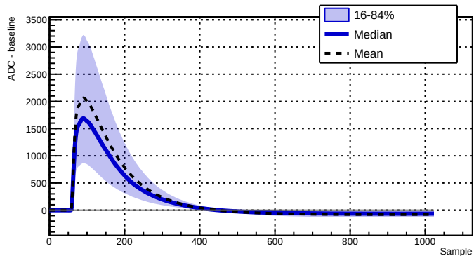
Run 039527 - Channel 2050 - 8860 waveforms
