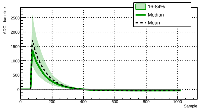
Run 043380 - Channel 2060 - 6067 waveforms
