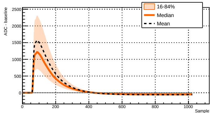
Run 043380 - Channel 2051 - 5860 waveforms
