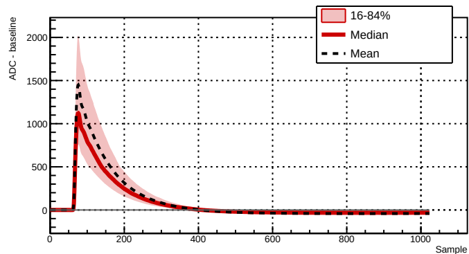
Run 043380 - Channel 2061 - 4862 waveforms
