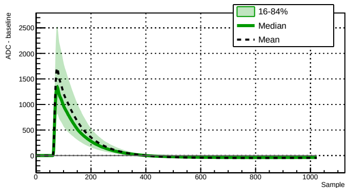
Run 043381 - Channel 2060 - 6040 waveforms
