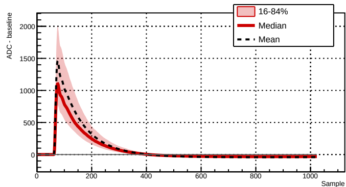
Run 043381 - Channel 2061 - 4993 waveforms
