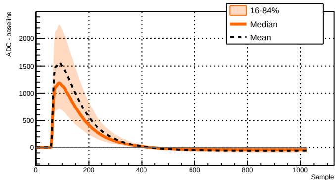
Run 043381 - Channel 2051 - 5939 waveforms
