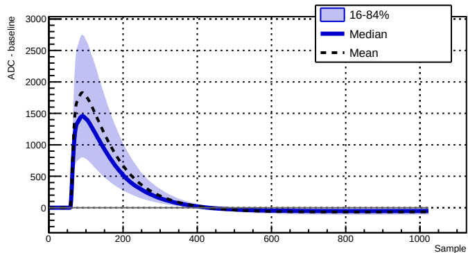
Run 043381 - Channel 2050 - 7380 waveforms
