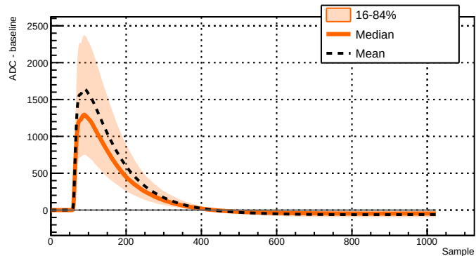
Run 043383 - Channel 2051 - 6347 waveforms
