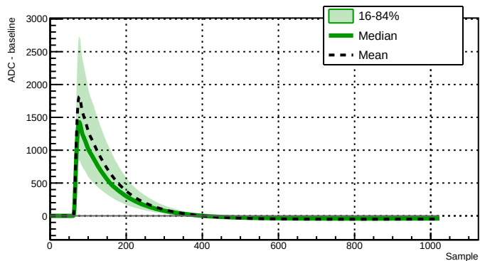
Run 043383 - Channel 2060 - 6278 waveforms
