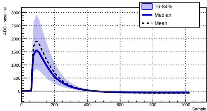
Run 043383 - Channel 2050 - 7954 waveforms
