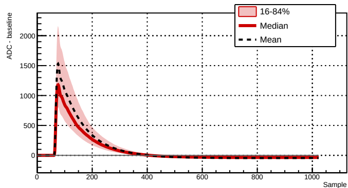
Run 043383 - Channel 2061 - 5158 waveforms
