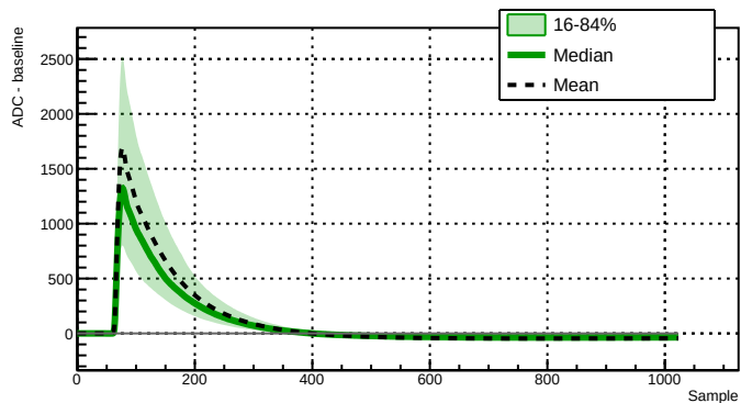
Run 043386 - Channel 2060 - 5953 waveforms
