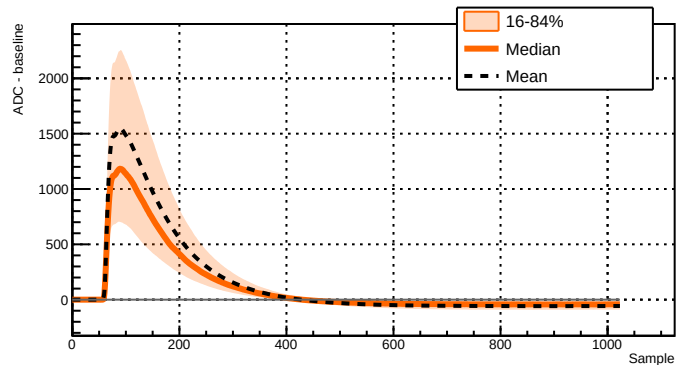
Run 043386 - Channel 2051 - 5718 waveforms
