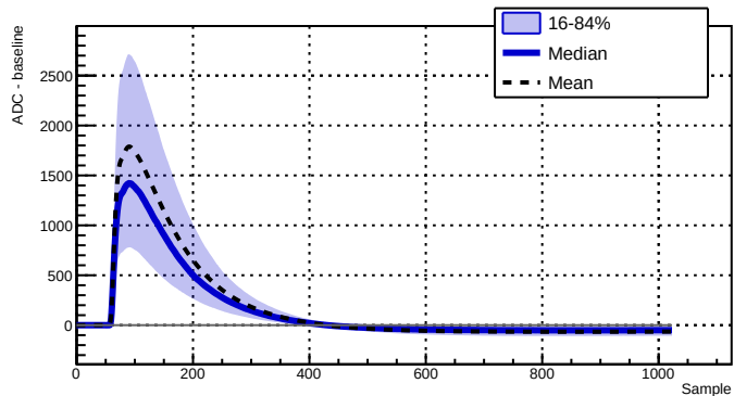
Run 043386 - Channel 2050 - 7332 waveforms
