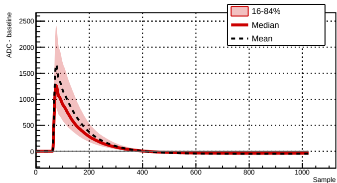
Run 043390 - Channel 2061 - 5360 waveforms
