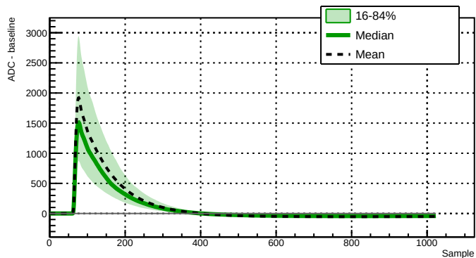
Run 043390 - Channel 2060 - 6748 waveforms
