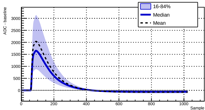
Run 043390 - Channel 2050 - 8540 waveforms
