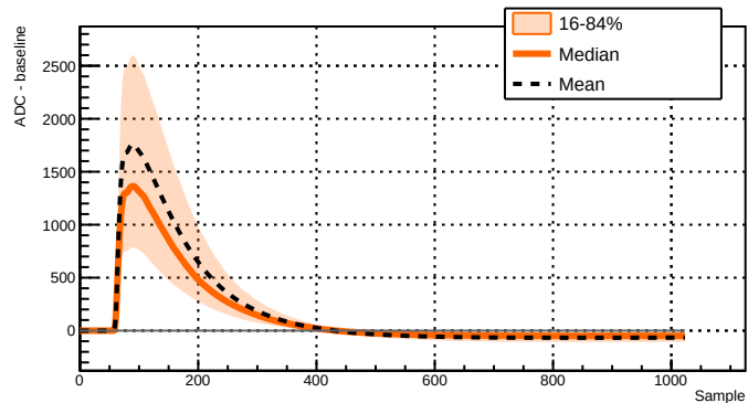
Run 043390 - Channel 2051 - 6863 waveforms
