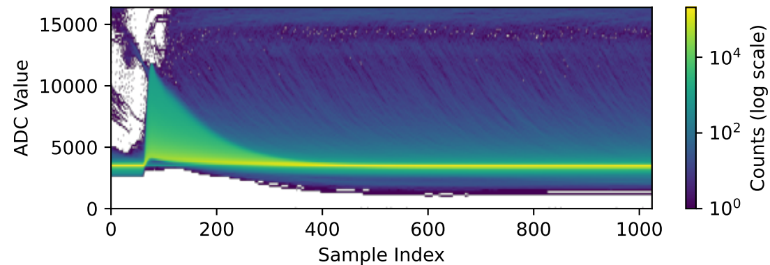
Channel 2070 (n=56144 waveforms)
