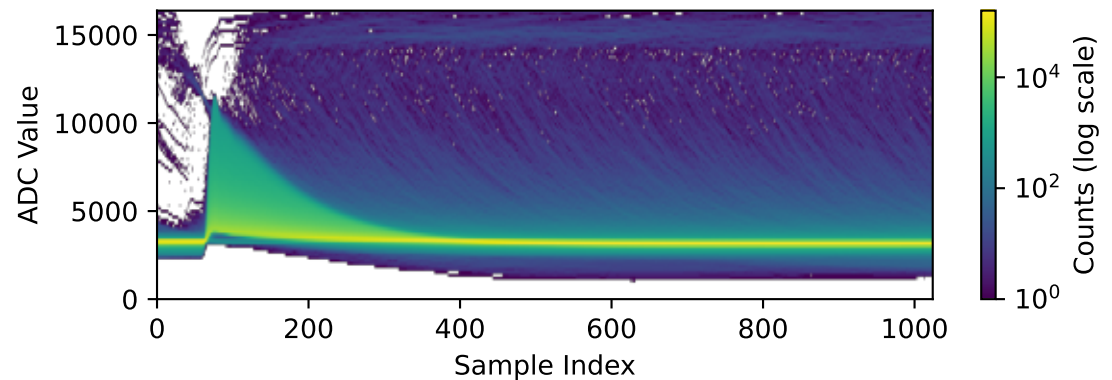
Channel 2071 (n=54848 waveforms)
