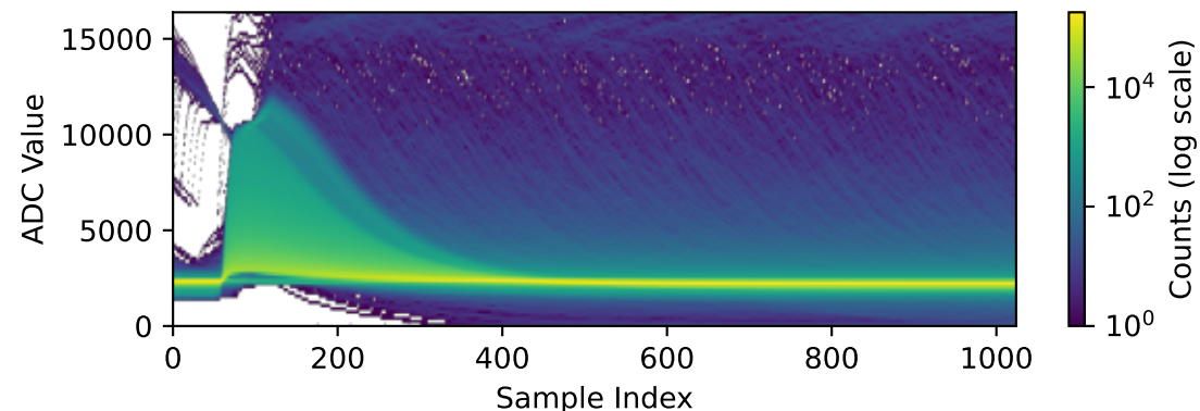
Channel 2080 (n=214511 waveforms)
