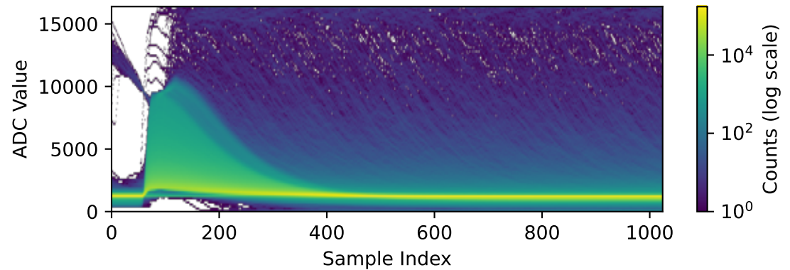
Channel 2061 (n=191356 waveforms)
