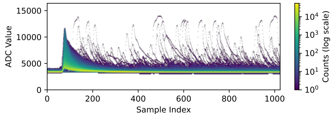
Channel 2081 (n=211331 waveforms)
