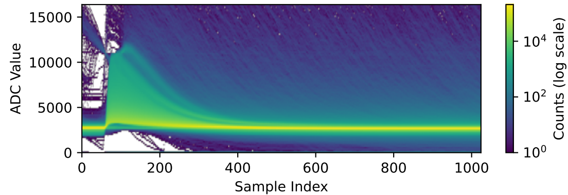
Channel 2050 (n=236646 waveforms)
