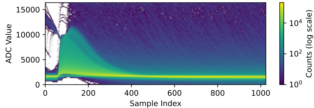
Channel 2060 (n=225867 waveforms)
