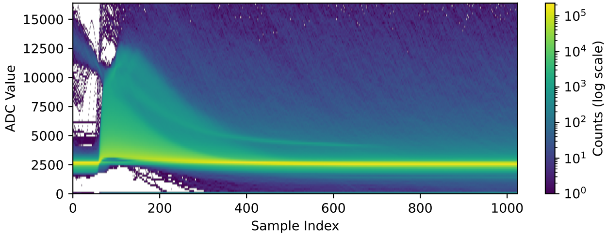
Channel 2031 (n=285397 waveforms)
