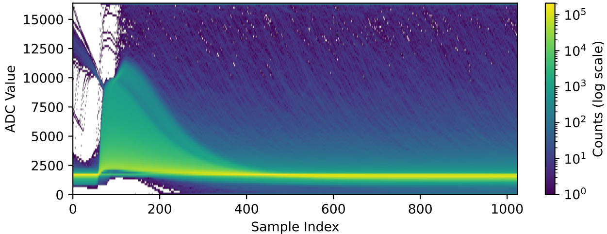
Channel 2050 (n=236646 waveforms)
