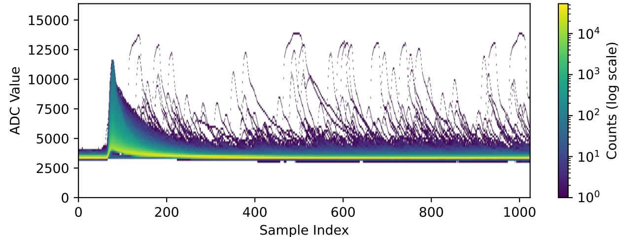
Channel 2071 (n=54848 waveforms)
