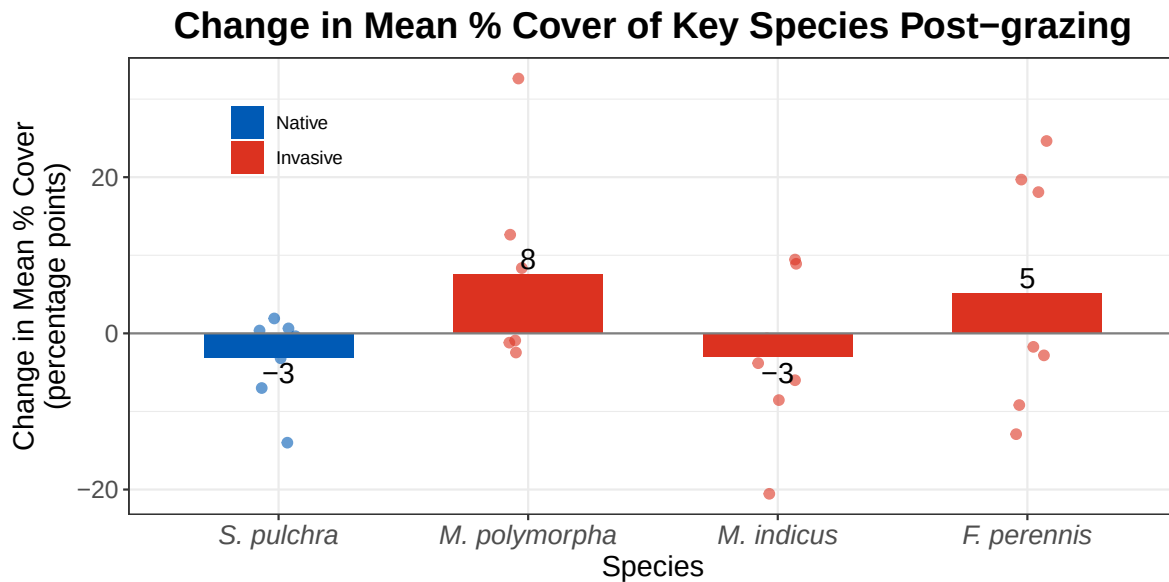
Figure 4: Change in mean percent cover of four key grassland species on the NCOS Mesa from 2024, pre-grazing, to 2025, post-grazing. Bars show the average percent-point change across transects, individual points show transect-level changes, and the gray horizontal line represents no change; blue indicates the native species Stipa pulchra , while red indicates invasive species. As an exploratory visualization, this figure suggests that S. pulchra changed only slightly after grazing, while invasive species showed mixed responses, with M. polymorpha and F. perennis increasing on average and M. indicus decreasing slightly.
