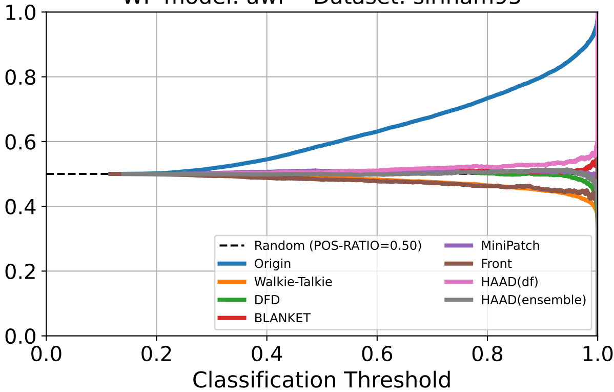
WF-model: awf Dataset: sirinam95
