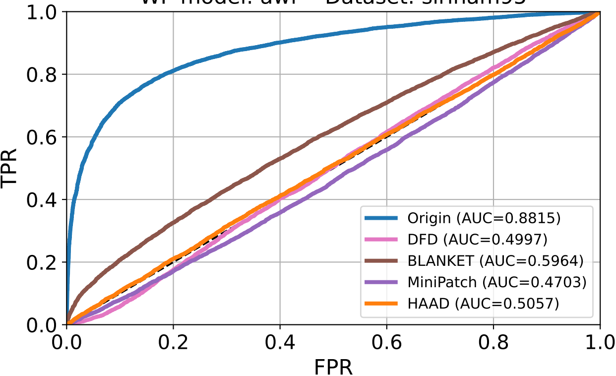
WF-model: awf Dataset: sirinam95
